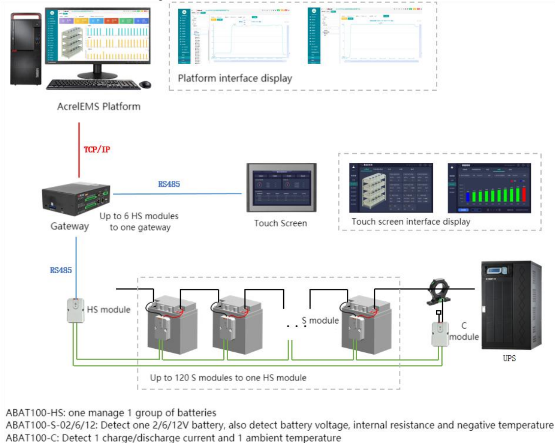
Fig.3 Network plan 2
