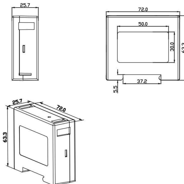
Fig.9 Dimensions of KDYA-DG1502-12K switching power supply
